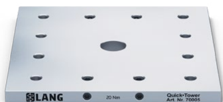
QUICK·TOWER BASE PLATE, THROUGH HOLE Ø 50H7, WITHOUT MOUNTING BORES
